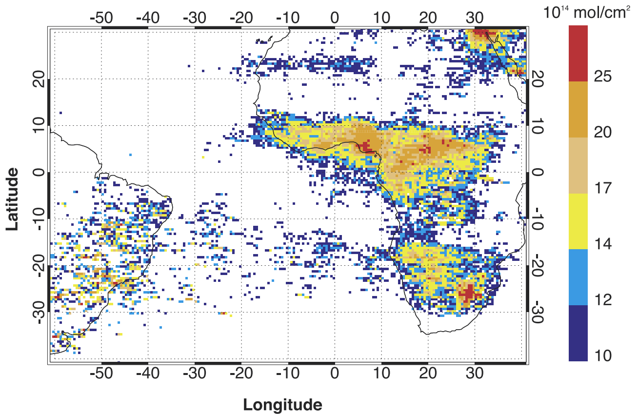
Figure 15. The January 2001 mean GOME residual tropospheric NO 2 vertical column. Data resolution is 0.5° longitude × 0.5° latitude.
