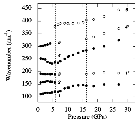
FIG. 2. Pressure-dependent evolution of the band position in the low- and mid-wave-number region (band 1 to 6) in the Raman spectra of \text{BaTi}_{0.65}\text{Zr}_{0.35}\text{O}_3 (BTZ 35 ).
