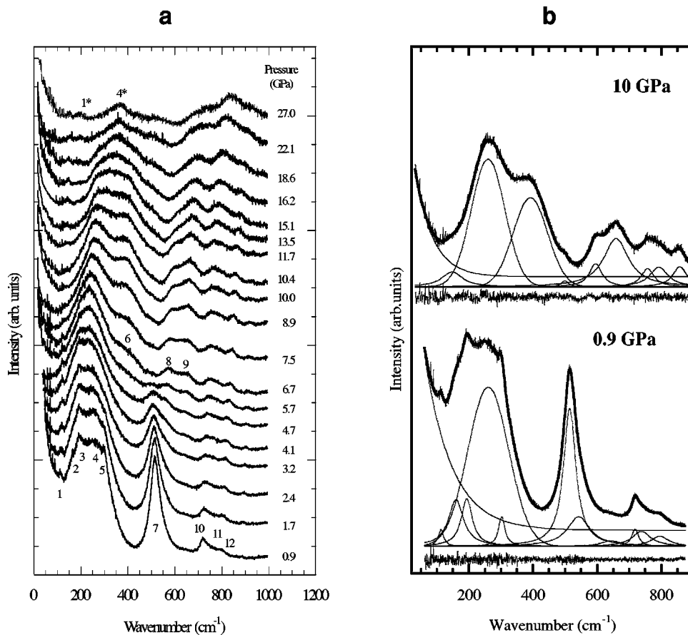
FIG. 1. (a) Representative pressure-dependent Raman spectra of \text{BaTi}_{0.65}\text{Zr}_{0.35}\text{O}_3 (BTZ 35 ). Modifications of the spectral signature (appearance/disappearance of bands, shift in wave number, etc.) reveal pressure-instabilities of BTZ 35 towards pressure. The band numbers are related to the notation introduced in the text. (b) Representative Lorentzian-shape deconvolution of Raman spectra at selected pressures.
