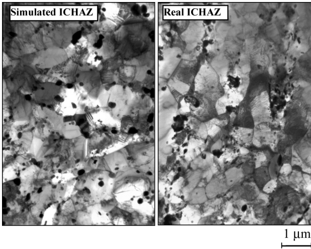
Fig. 6. Thin foil TEM investigations: Comparison of real and simulated intercritical heat affected zone ( T_{peak}=986^{\circ}\text{C} ) microstructures (bright field images).
