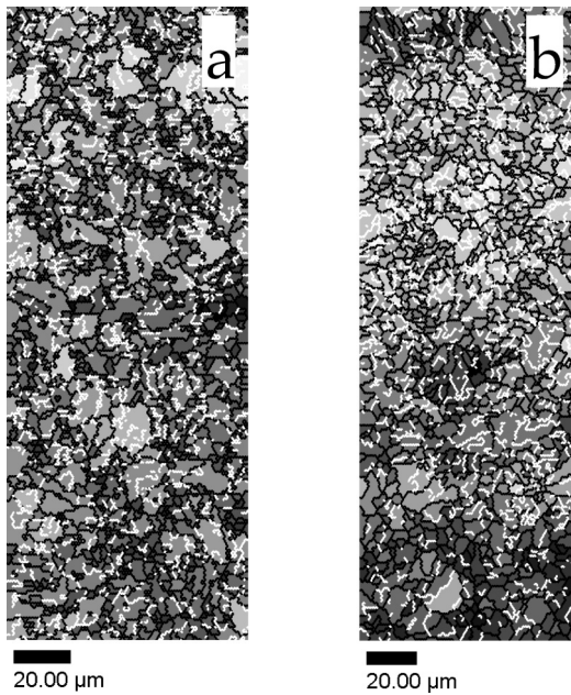
Fig. 7. EBSD investigations of (a) real and (b) simulated intercritical heat affected zones ( T_{peak}=986^{\circ}\text{C} ). White (resp. black) lines delineate low angle ( 5-15^{\circ} ) boundaries (resp. high-angle boundaries >15^{\circ} ).
