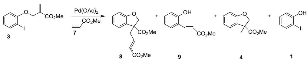
Scheme 4. Pd-catalyzed tandem cyclization/Heck reaction.
