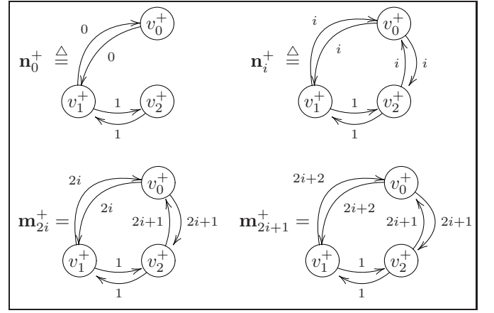
Fig. 10. Example of an infinite strictly increasing chain defined by \mathbf{m}_0^+ = (\mathbf{n}_0^+)^\bullet , \mathbf{m}_i^+ = (\mathbf{m}_{i-1}^+ \nabla ((\mathbf{n}_i^+)^\bullet))^\bullet . Remark that the nodes \{v_0^-, v_1^-, v_2^-\} are not represented here due to lack of space; this part of the DBMs can be easily figured out by coherence.
