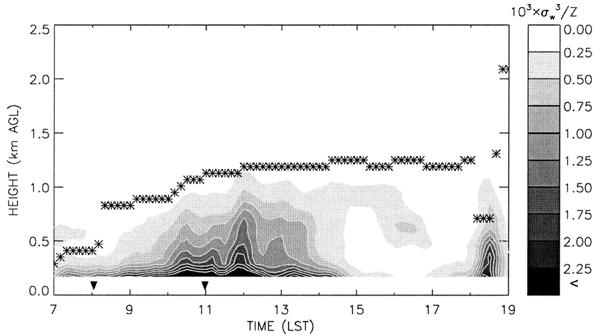
FIG. 8. Time-height cross section of \sigma_w^3/z with the CBL heights (asterisks) estimated by the new method using C_n^2 and \sigma_w for 19 Jun 1998 at Viabon.
