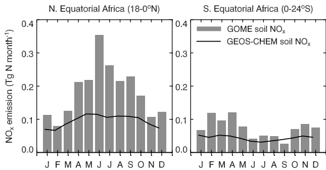
Figure 5. Seasonal variation in soil \text{NO}_x emissions for north equatorial Africa ( 18\text{--}0^\circ\text{N} ) and south equatorial Africa ( 0\text{--}24^\circ\text{S} ) in 2000. The gray bars show the monthly top-down GOME soil \text{NO}_x emissions. The solid line represents the GEOS-CHEM soil emission inventory based on Yienger and Levy.
