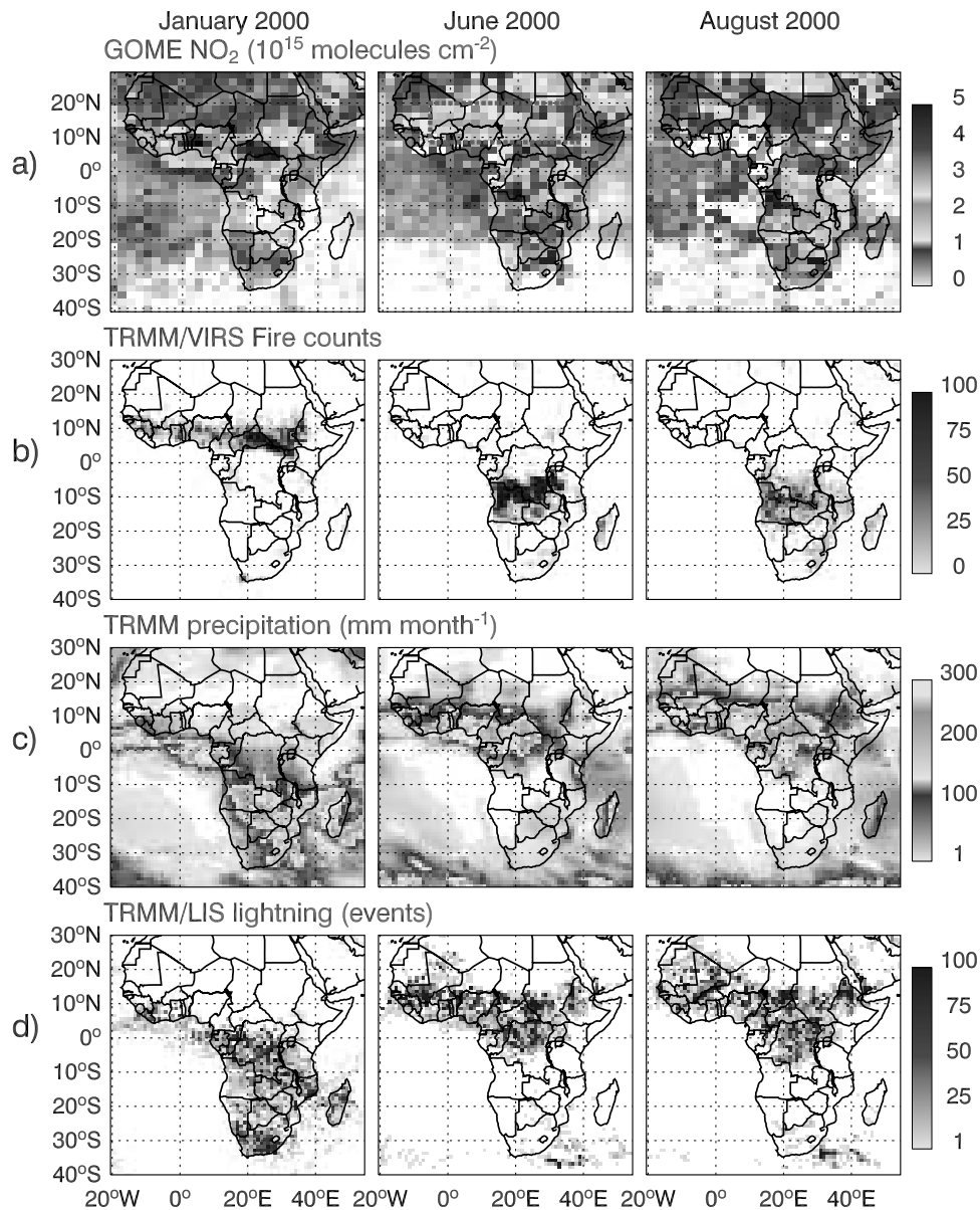
Figure 1. Space-based observations of \text{NO}_2 columns, fires, precipitation and lightning over Africa for January, June, and August 2000. (a) Monthly mean GOME \text{NO}_2 tropospheric columns in 10^{15} molecules \text{cm}^{-2} . (b) Total active fires observed by the Visible and Infrared Scanner (VIRS) on board the TRMM satellite. (c) Monthly precipitation from the TRMM merged analysis in \text{mm month}^{-1} . (d) Monthly lightning activity from the lightning imaging sensor (LIS) on board TRMM. GOME observations are averaged over a 2^\circ latitude by 2.5^\circ longitude horizontal grid, while all TRMM observations are averaged over a 1^\circ \times 1^\circ grid. The \text{NO}_2 enhancements over the Sahel region during June are highlighted with a dotted rectangle in the top panel. See color version of this figure at back of this issue.
