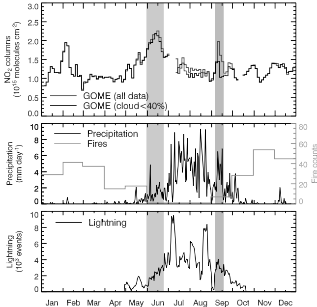
Figure 2. Evolution of \text{NO}_2 , precipitation and fires over 1.5 million \text{km}^2 of the southern Sahel ( 12\text{--}16^\circ\text{N} ; 0\text{--}30^\circ\text{E} ). (top) Time series of 3-day composite tropospheric GOME \text{NO}_2 columns averaged over the southern Sahel. All data (red) as well as cloud-filtered data (black, <40\% cloud cover) are shown. A 9-day running average was used to smooth the observations. Gaps indicate 6 days or more without observations. (middle) TRMM daily precipitation (black line) and monthly fire counts (orange line). (bottom) TRMM/LIS lightning events. The green shading indicates the June soil \text{NO}_x pulse, while the gray shading shows a later pulse in September (section 3). See color version of this figure at back of this issue.
