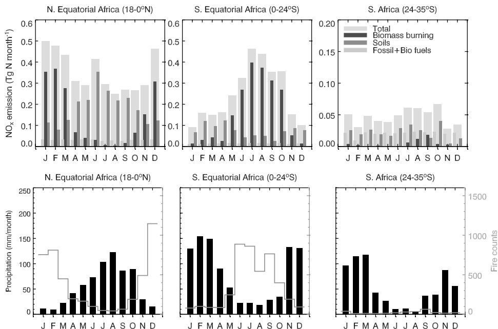
Figure 4. Monthly \text{NO}_x emissions, fires and rainfall over north equatorial Africa ( 18-0^\circ\text{N} ), south equatorial Africa ( 0-24^\circ\text{S} ) and southern Africa ( 24-35^\circ\text{S} ) in 2000. (top) Monthly top-down GOME \text{NO}_x emissions averaged over each region (gray bars). Note the different scale on the right-most panel. We combine bottom-up estimates of biofuel and fossil fuel \text{NO}_x emission inventories with the spatial location of fires to partition emissions between biomass burning (red bars), soil (blue bars), and fossil+biofuel (green bars) sources. (bottom) Seasonal variations in total active fires (solid orange line) and mean precipitation (black bars) observed by TRMM. See color version of this figure at back of this issue.
