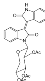
Natura 1-(β-D- O -triacetyloxylopyranosyl)-isoindigo
