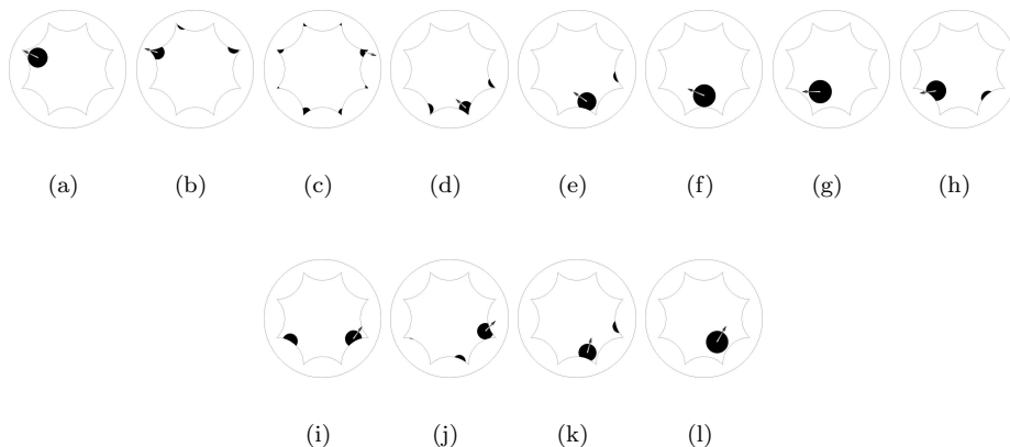
Figure 17. Successive snapshots of the trajectory of a single disk-like particle freely evolving on the pseudosphere in the Poincaré representation, with the periodic boundary condition shown in figure 7(a). The trajectory follows geodesics, i.e. , circular arcs and the arrow indicates the direction of motion. Note the complex pattern of exits and reentries. The fact that the particle is not considered as a mere point but has a finite size makes the pattern even more intricate.
