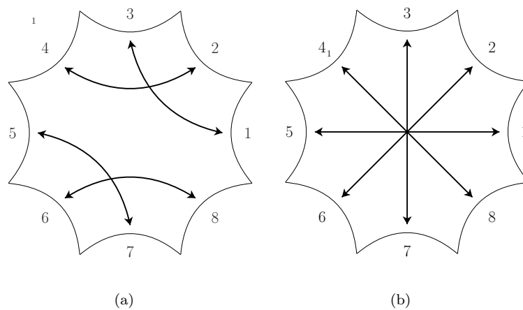
Figure 7. Fundamental polygons corresponding to the decorated graphs of figure 6: (a) corresponds to figure 6(a) and (b) to figure 6(b). The pairings are the only ones allowed for the \{8, 8\} tiling of H^2 .
