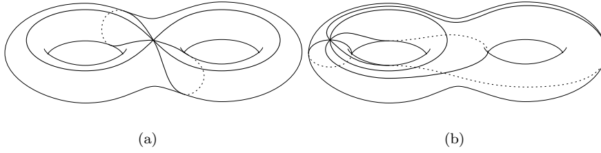
Figure 9. Compact manifold and graphs obtained by gluing the edges of the fundamental polygons of figure 7(a) (in(a)) and figure 7(b) (in (b)). The graphs embedded in the compact manifold (a two-hole torus) correspond to the planar representations of figure 6.
