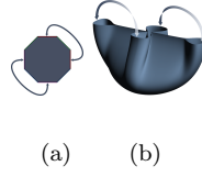
Figure 8. Schematic representation of the “compactification” of the fundamental polygon shown in figure 7(a). The paired edges are glued together: 1 with 3 and 5 with 7 in (a); 2 with 4 and 6 with 8 in (b). The final compact manifold is a two-hole torus represented in figure 9(a).
