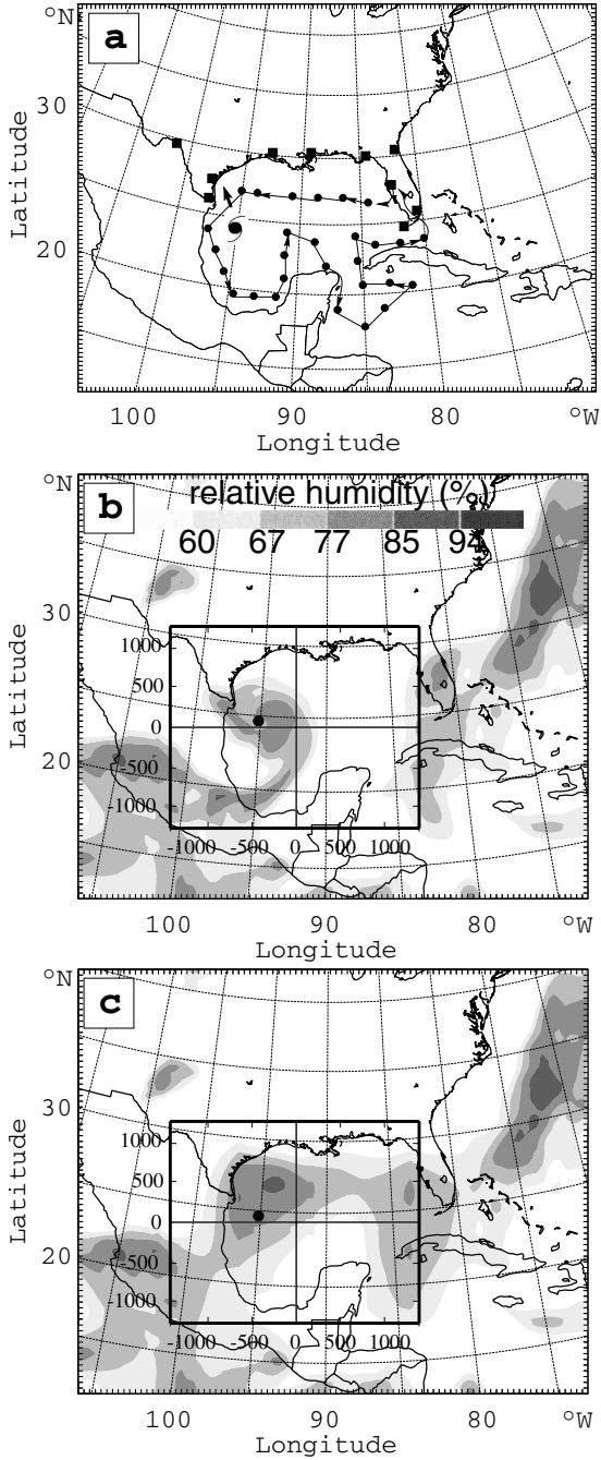
Figure 5. (a) Omega dropsonde sampling from the NOAA Gulfstream IV-SP aircraft from 1751 UTC 21 August to 0143 UTC 22 August (black squares) and location of radiosoundings available at 00 UTC 22 August near the Gulf of Mexico (black dots); (b) mid-tropospheric (700–400 hPa) relative humidity (%), from the ECMWF global analysis at 0000 UTC 22 August; (c) mid-tropospheric relative-humidity field from a modified analysis including the data from OMEGA dropsondes.
