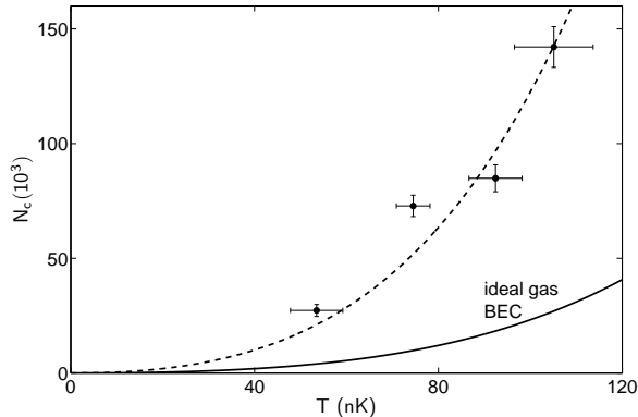
Figure 4: Critical point in an interacting 2D gas. The critical atom number N_c ( \bullet ) is measured at four different temperatures T . Displayed error bars are statistical. The solid line shows the ideal 2D gas BEC prediction N_{c,id}^{multi} . The dashed line is the best empirical fit to the data, which gives N_c = \alpha N_{c,id}^{multi} with \alpha = 5.3(5) .
