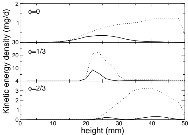
Fig. 11. Division of kinetic energy into mean motion ( “hydrodynamic”) and disorganized parts ( “thermal”) as a function of altitude at 3 different phases \phi of the vibrating cycle. ( \cdots ) Thermal kinetic energy (data for V = 3 from Fig. 10). (—) Hydrodynamic kinetic energy, obtained by averaging the velocities of all particles found in each strip.
