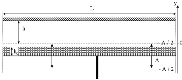
Fig. 2. Typical aspect ratio of the container for n = 5 layers of particles (2 mm in diameter) leading to a height of the bed of particles at rest, h_0 = 1 cm. The container height is h = 2.5 cm, its length L = 20 cm, and the peak-peak vibrational amplitude A = 2.5 cm (see text for details).
