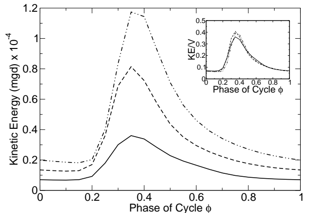
Fig. 9. Total kinetic energy of the particles as a function of vibration phase \phi for three different velocities V = 1, 2 and 3 m/s (from lower to upper) at constant number of particles n = 5 . The wall is at its lowest at \phi = 0 and \phi = 1 , and reaches its highest point at \phi = 0.5 . Data from 100 cycles were averaged to obtain these curves. Inset: Total kinetic energy rescaled by V as a function of \phi .
