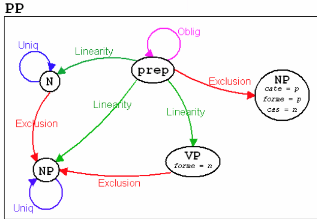
figure 1 : Constraint graph of the Prepositional Phrase (PP)
