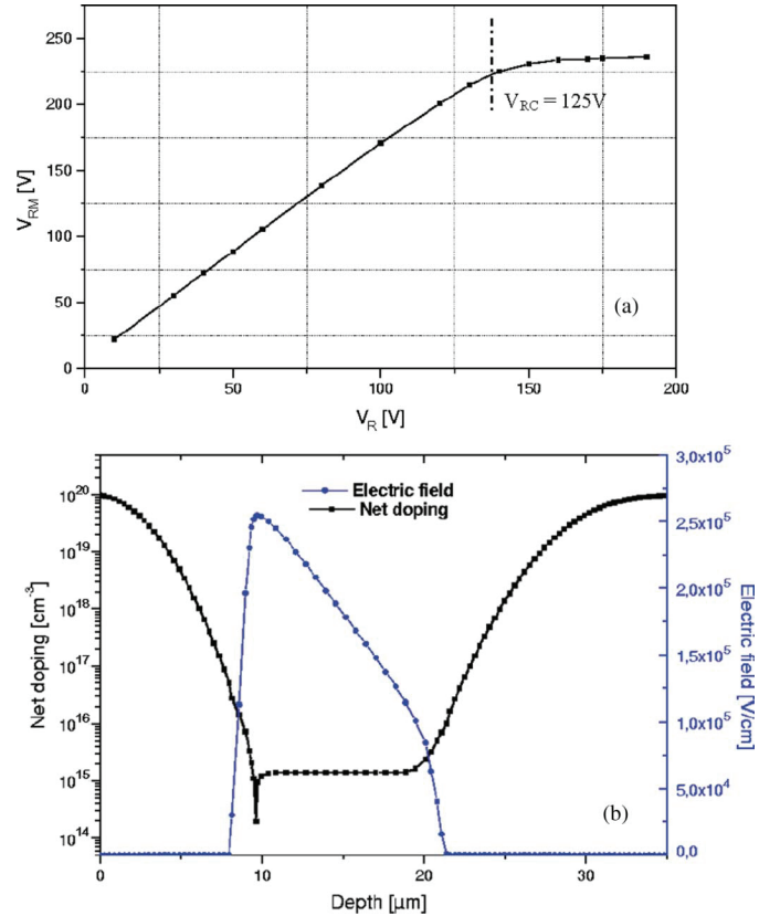
Fig. 9. Results for the device BYW81P200. (a) Experimental V_{RM} versus V_R . V_{BR} = 230 V and V_{RC} = 125 V ( V_{BR} = 200 V in datasheet). (b) Simulated electric field distribution at onset of avalanche ( V_R = 200 V).
