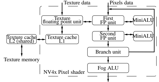
Figure 3. Pixel shader of the Nvidia 7800GTX.
