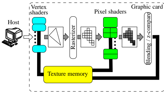
Figure 1. Model of the graphics pipeline.
