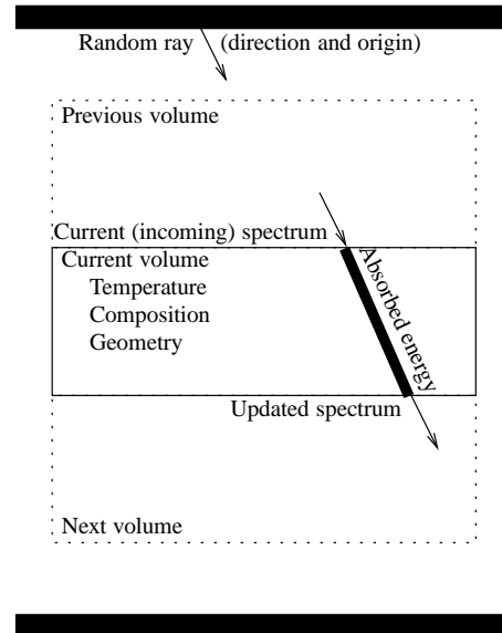
Figure 5. Monte-Carlo ray-tracing.
