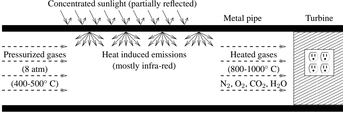
Figure 4. The solar receptor as simulated.
