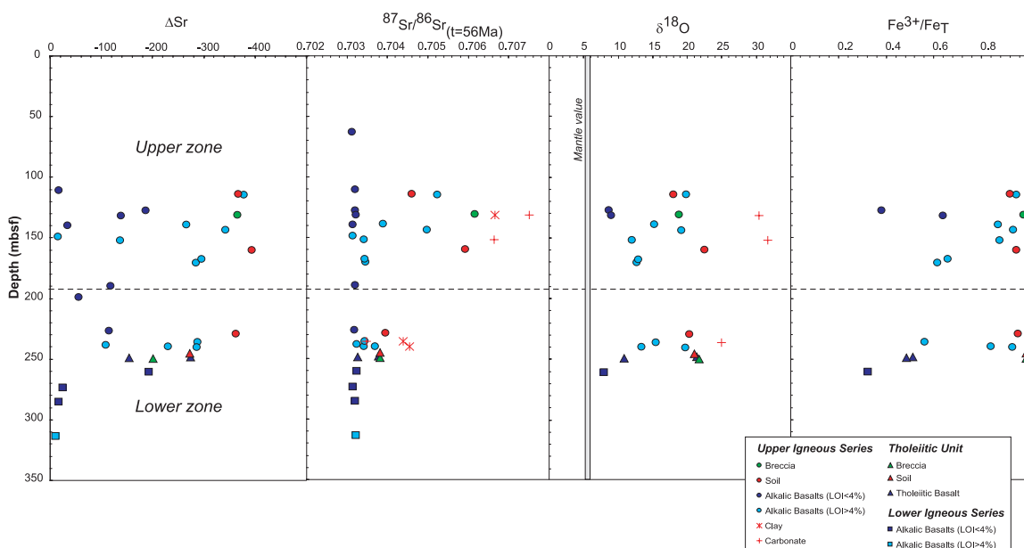
Figure 8. \Delta\text{Sr} , ^{87}\text{Sr}/^{86}\text{Sr}_{(56\text{ Ma})} , \delta^{18}\text{O} (‰), and \text{Fe}^{3+}/\text{Fe}_T versus depth (mbsf) of some fresh and altered samples from Hole 1205A. Sr and O isotopes compositions of separated clay and carbonate minerals are also plotted. \Delta\text{Sr} (ppm) is calculated as [\text{Sr}]_{\text{altered sample}} - [\text{Sr}]_{\text{protolith}} .
