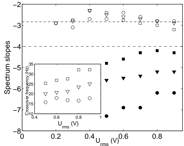
FIG. 4: Slopes of surface-height spectra for gravity (full symbols) and capillary (open symbols) waves for different forcing band widths and intensities: ( \circ ) 0 to 4 Hz, ( \nabla ) 0 to 5 Hz and ( \square ) 0 to 6 Hz. Power-law exponents of gravity wave spectrum ( - ) and capillary waves spectrum ( - ) as predicted by WT theory (Eq. 1). Inset: Cross-over frequency between gravity and capillary regimes as a function of the forcing intensity and band width.
