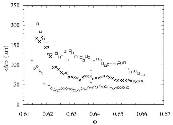
FIG. 4: Evolution of the mean step size \langle \Delta r \rangle with \Phi during compaction for \theta = 2.7^\circ (o); \theta = 5.4^\circ (x); \theta = 8.4^\circ ( \square ). The average \langle \rangle means over 40 identical slots in \Phi and over particles. Fluctuations from one particle to another due to heterogeneities in the packing and force network are given by the error bar.
