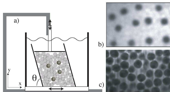
FIG. 1: a) Experimental setup. b) Picture of the packing full of index matching liquid with 12 colored tracers. The fuzziness allows a better accuracy for particle tracking. c) Picture obtained with the laser sheet method.
