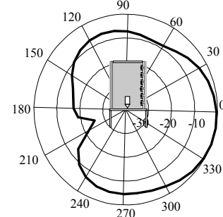
Fig.15 – Simulated radiation patterns in the E plan at 0.94GHz.
