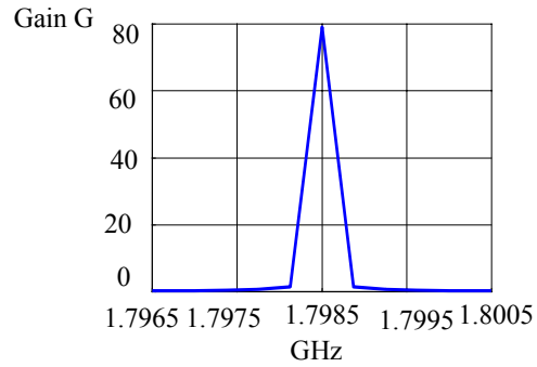
Figure 6 : (a) : Gain and envelop ( D=41.7mm , P_t=0.9mm , a=0.36mm ) (b) : zoom on the transmission pick.
