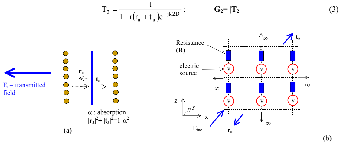
Figure 7 : (a) : Antenna interacting with cavity waves (b) : Antenna model composed of an infinite plane of point voltage sources in series with point resistances ( \mathbf{R} )
