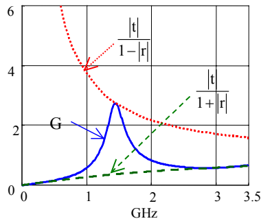
Figure 4 : Maximum and minimum envelopes ( D=40mm , P_t=40mm , a=2mm )
