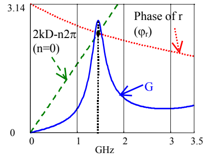
Figure 5 : Determination of the transmission pick frequency. ( D=40mm , P_t=40mm , a=2mm )
