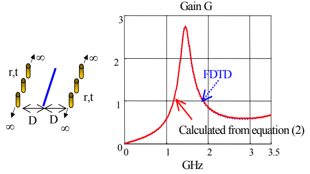
Figure 3 : Gain enhancement G . Comparison between FDTD method and formula (2) ( D=40mm , P_t=40mm , a=2mm )
