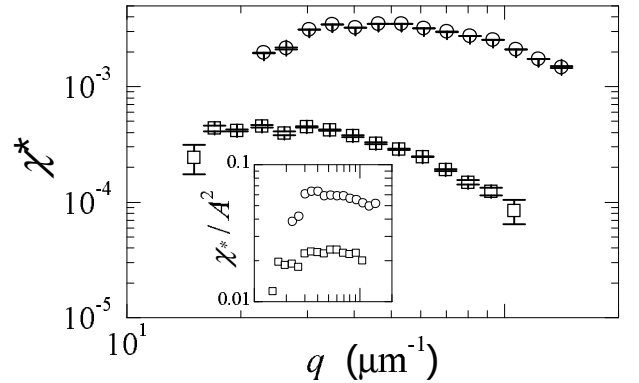
FIG. 5: Peak of the dynamic susceptibility, \chi^* , vs q for a CB gel with 0.2% dispersant (squares) and no dispersant (circles). Error bars are calculated as explained in sec. II. Inset: same data normalized by the squared amplitude of g_2 - 1 .
