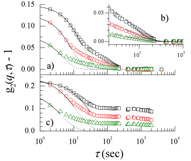
FIG. 4: (Color online) a): Intensity correlation functions representative of the behavior at small, intermediate and large q vectors for the CB gel with 0.2% dispersant (symbols; from top to bottom, q = 17.1, 39.6 , and 80.8 \mu\text{m}^{-1} ). The lines are fits to the initial decay of g_2 - 1 issued from the scaling analysis described in the text. b): zoom on the final decay of g_2 - 1 for the same data as in a), together with the large- \tau fits (lines). c): g_2 - 1 vs \tau for the CB gel with no dispersant (symbols; from top to bottom, q = 26.5, 61.2 , and 141.5 \mu\text{m}^{-1} ). In a) and c) the fits are represented as solid lines for \tau \leq \tau_1 and continued as dashed lines beyond the fitting interval.
