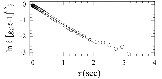
FIG. 1: Second-order cumulant fit (line) of the intensity correlation function (open circles) measured by dynamic light scattering at q = 6.01 \mu\text{m}^{-1} for a diluted suspension of CB particles.
