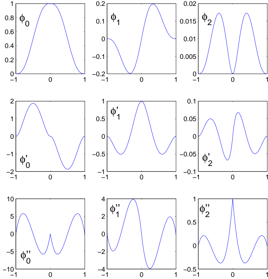
Figure 1: Basic Hermite interpolation functions and their derivatives of order 1 and 2 in the Hermite interpolation scheme of degree 2
