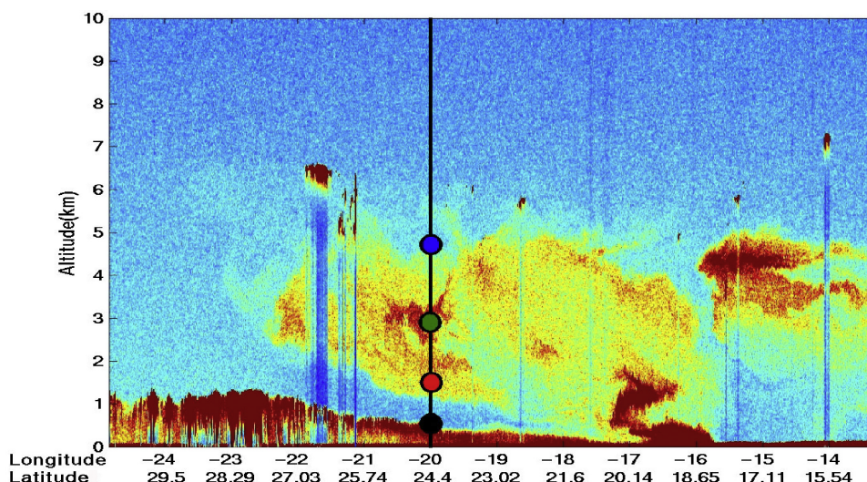
Figure 2. Raw LITE data of orbits 115 for 17 September 1994. The orbit crosses the northern Mauritanian coast at about 20^{\circ}\text{N} . A dust uptake seems to occur between 18.5 and 20^{\circ}\text{N} . The marine atmospheric boundary layer is very shallow close to the coast but reaches more than 1 km in the northwest of the dust plume area. Colored circles mark the starting points of back trajectories shown in Figure 1.
