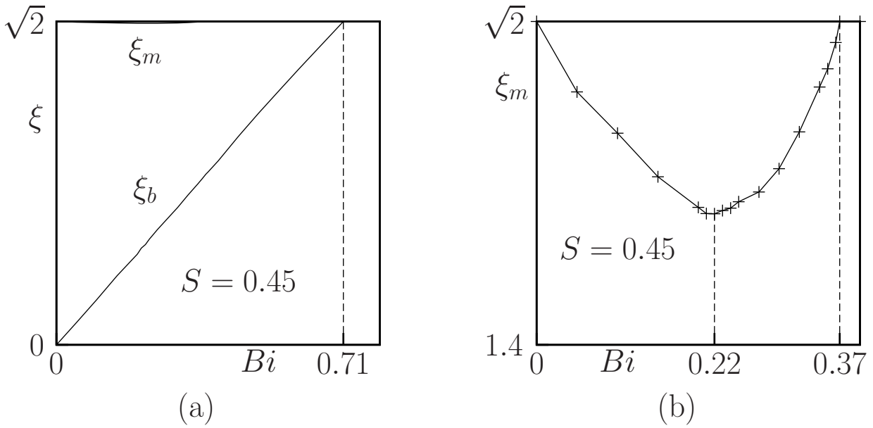
Figure 15. Position on the square diagonal of the rigid zones boundaries as functions of Bi , for S = 0.45 : position \xi_m for the dead zones and \xi_b for the plug: (a) curves (Bi; \xi_m(Bi)) and (Bi; \xi_b(Bi)) ; (b) zoom on the curve (Bi; \xi_m(Bi)) .
