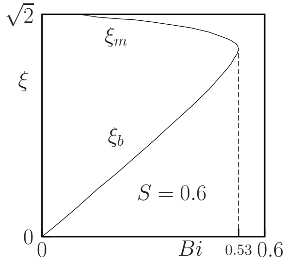
Figure 9. Position on the square diagonal of the dead zone boundary \xi_m and the plug boundary \xi_b , as functions of Bi , with S = 0.6 .
