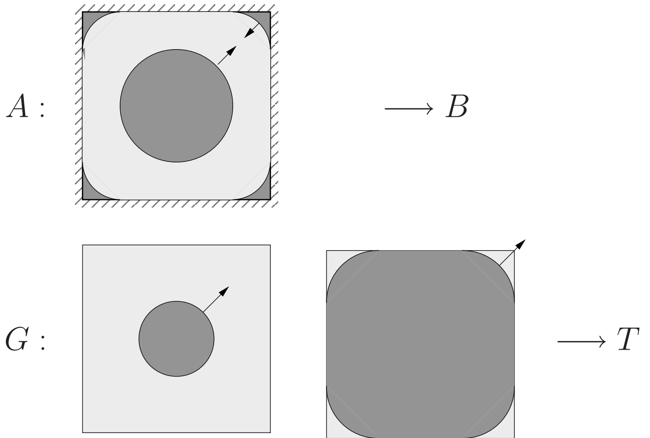
Figure 20. Schematic representation of the flow in the regimes A and G when Bi increases: evolution of the rigid zones boundaries and of the stick-slip transition points.
