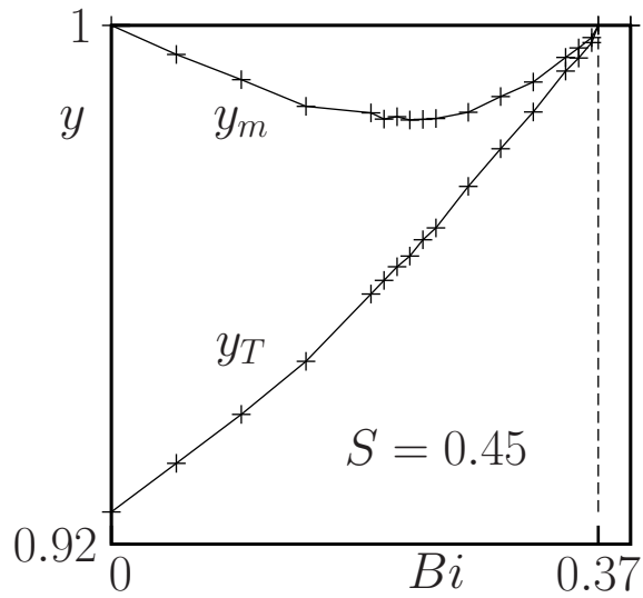
Figure 17. Position at the wall of the free boundaries as functions of Bi for S = 0.45 : position y_m of the dead zone boundary, position y_T of the stick-slip transition.
