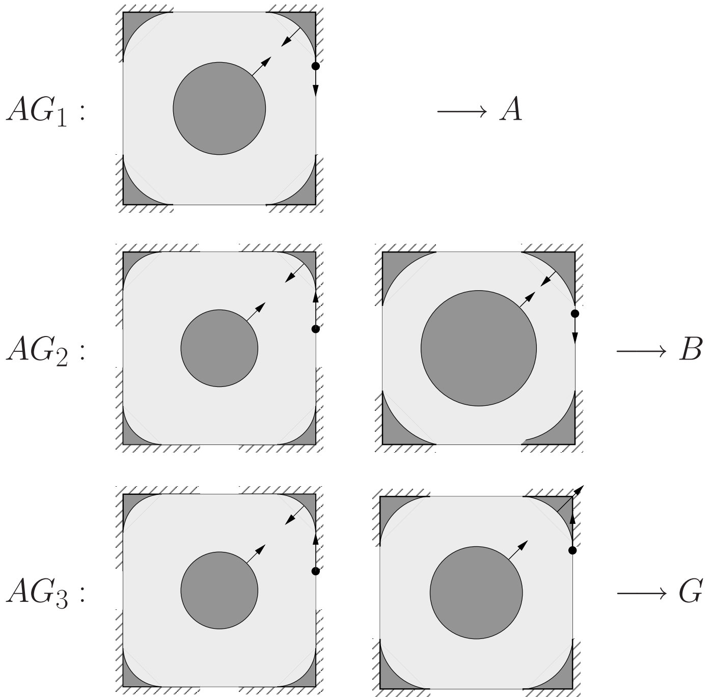
Figure 21. Schematic representation of the flow in the sub-regimes AG_1 , AG_2 and AG_3 when Bi increases: evolution of the rigid zones boundaries and of the stick-slip transition points.
