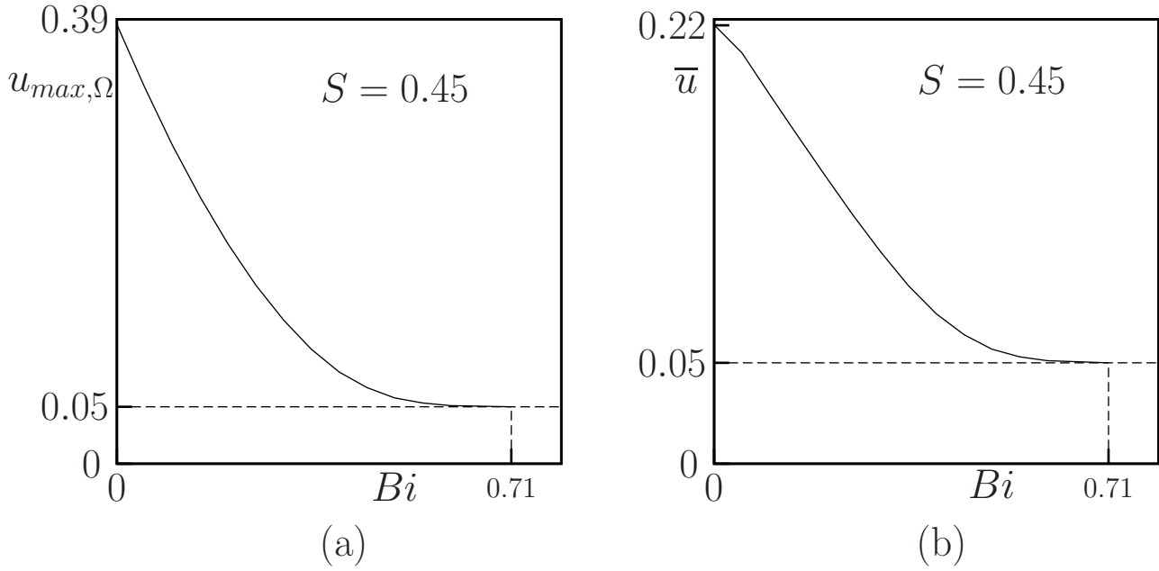
Figure 14. (a) Maximum velocity u_{max,\Omega} versus Bi for S = 0.45 . (b) Flow rate \bar{u} versus Bi , for S = 0.45 .
