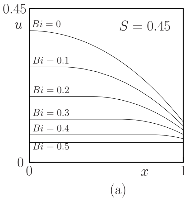
Figure 11. Velocity profiles for some values of Bi and S = 0.45 : (a) cut along the horizontal axis ; (b) cut along the diagonal.
