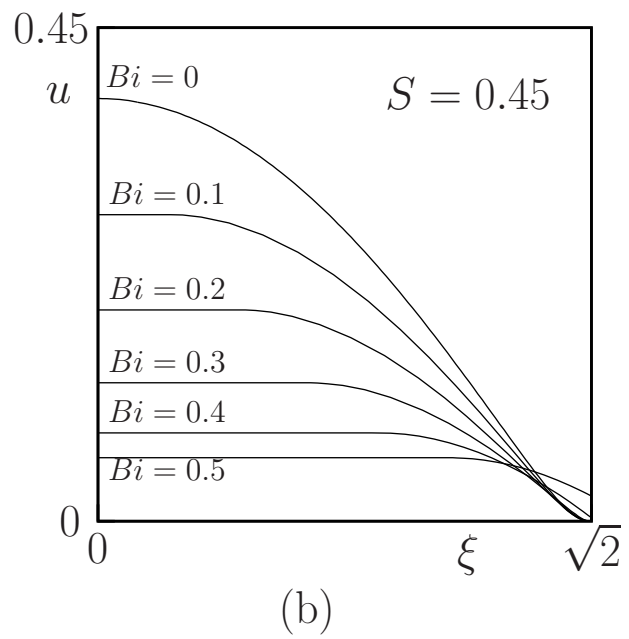
Figure 11. Velocity profiles for some values of Bi and S = 0.45 : (a) cut along the horizontal axis ; (b) cut along the diagonal.
