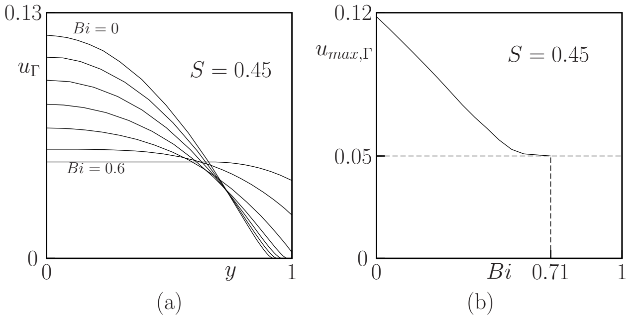
Figure 16. Velocity at the wall for S = 0.45 (mixed regime where both stick and slip exist): (a) for Bi \in \{0; 0.1; 0.2; 0.3; 0.4; 0.5; 0.6\} ; (b) maximum value versus Bi .
