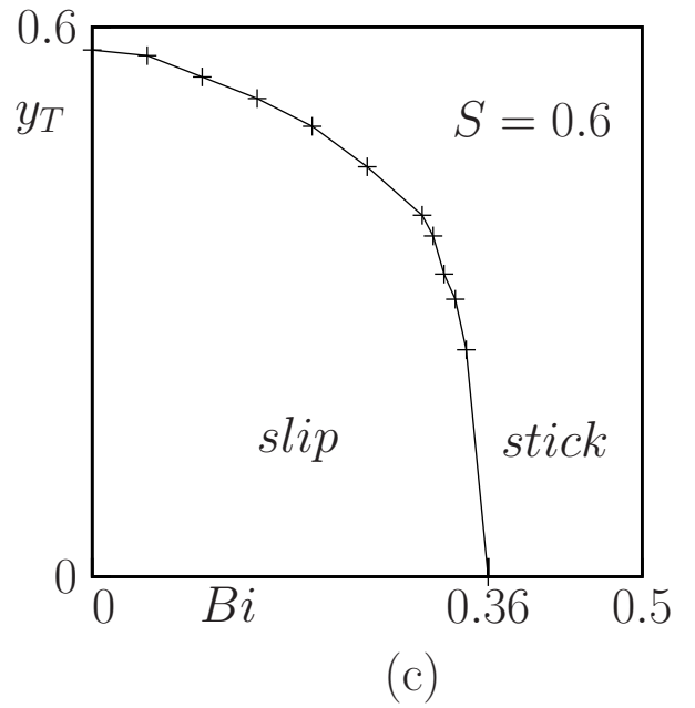
Figure 5. Velocity at the wall for S = 0.6 : (a) dependence upon Bi ; (b) intersection with the y -axis: maximum wall velocity versus Bi ; (c) intersection with the x -axis: coordinate y_T of the stick-slip transition point as a function of Bi .
