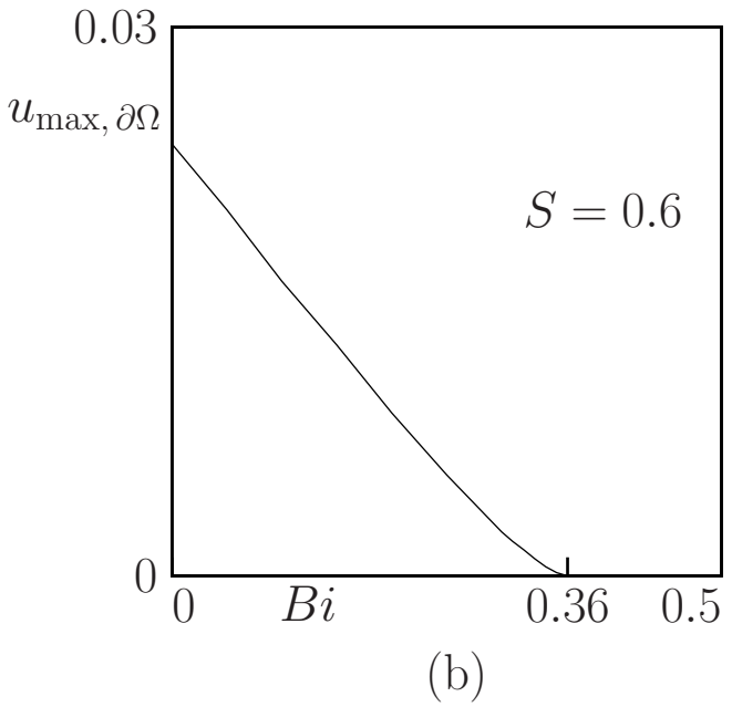
Figure 5. Velocity at the wall for S = 0.6 : (a) dependence upon Bi ; (b) intersection with the y -axis: maximum wall velocity versus Bi ; (c) intersection with the x -axis: coordinate y_T of the stick-slip transition point as a function of Bi .
