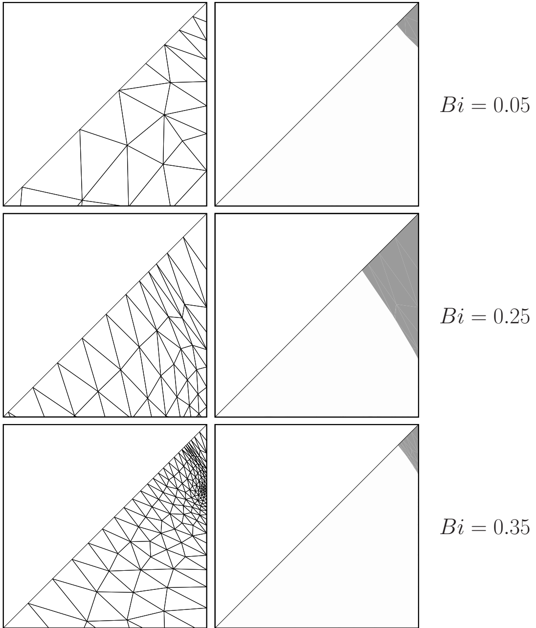
Figure 13. Adapted meshes and associated solutions, zoomed in the corner ( 0.98 \leq y \leq 1 ) for S = 0.45 : rigid zones in dark gray, deforming zones in light gray.
