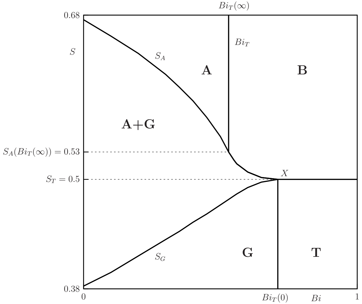
Figure 18. The main flow regimes for a square section: curves (Bi; S_A(Bi)) , (Bi; S_G(Bi)) and (Bi_T(S); S) , and value S_T separating the regimes; particular point X and values Bi_T(0) , Bi_T(\infty) and S_A(Bi_T(\infty)) ; representation in dashed lines of the values of S used to study the dependence of the flow upon Bi .
