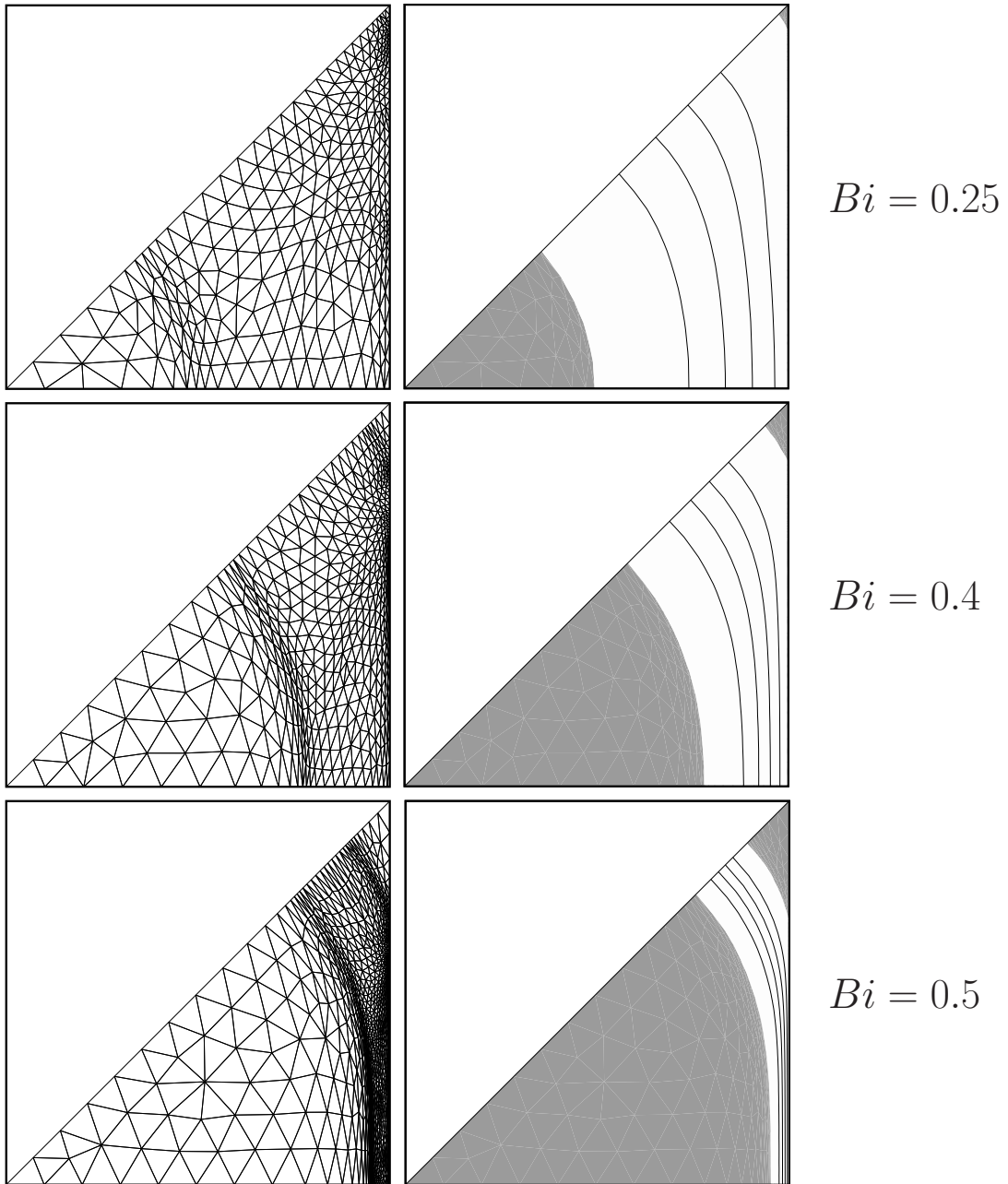
Figure 8. Adapted meshes and their associated solutions for S = 0.6 : rigid zones in dark gray, deforming zones in light gray, and isovalues of the velocity.
