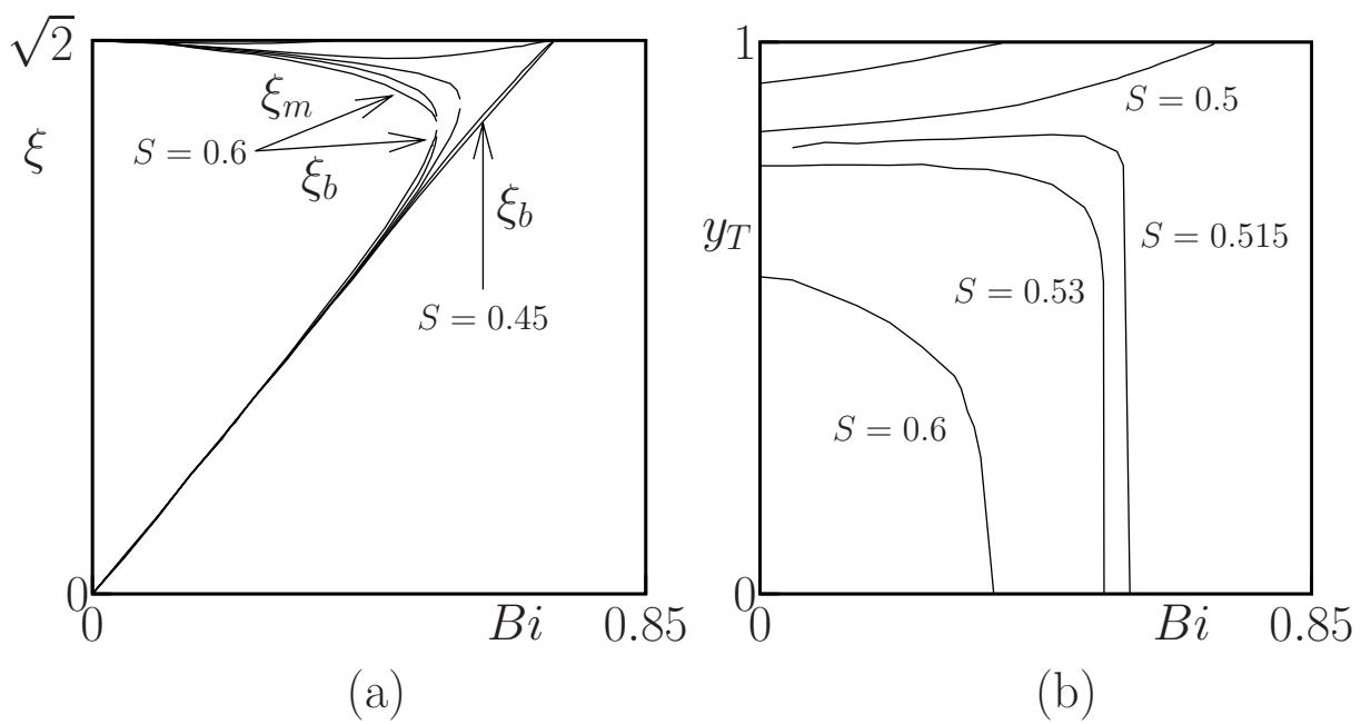
Figure 19. Evolution of the free boundaries versus Bi , for some values of S : (a) positions \xi_m of the dead zone and \xi_b of the plug along the square diagonal ; (b) position y_T of the stick-slip transition point.
