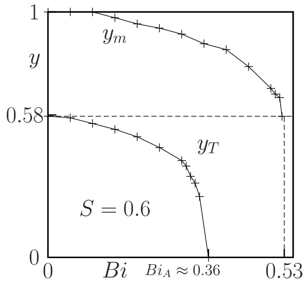
Figure 10. Positions on the wall of the free boundaries, as functions of Bi , with S = 0.6 : position y_T of the stick-slip transition point, position y_m of the dead zone boundary.
