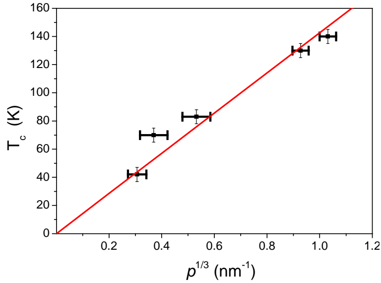
Fig. 1: (Color online) Curie temperature as a function of p^{1/3} where p is the mean hole density between n=1 and n=2 fit results (given by the tips of the horizontal bars). Full line is the fit to the mean-field expression T_c \propto p^{1/3} .
