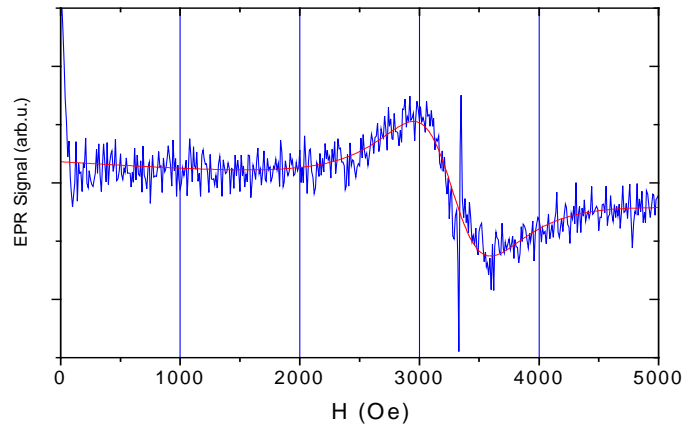
Fig. 5: EPR spectrum of the fully passivated sample; T=20\text{K} . The sharp line at 3300 Oe is a surface signal.
