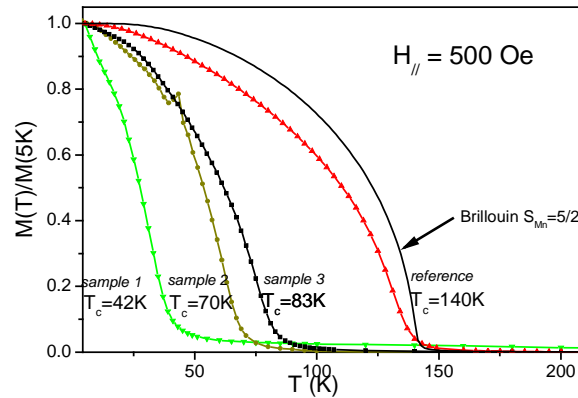
Fig. 2: (Color online) Temperature-dependence of the normalized magnetization under a 500 Oe in-plane field for samples 1-3, and reference. The solid line corresponds to Brillouin curve with S_{Mn} = 5/2 , and T_c = 140 K. Curie temperatures increase and curves become more convex with increasing hole density.
