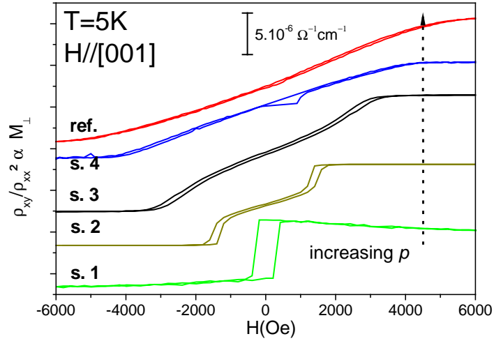
Fig. 4: (Color online) Hysteresis cycles obtained by anomalous Hall effect 25 with H//[001] (off-set for clarity), and assuming M_{\perp} \propto \rho_{xy}/\rho_{xx}^n with n=2 . The magnetic easy axis flips from out-of-plane to in-plane with increasing hole density.
