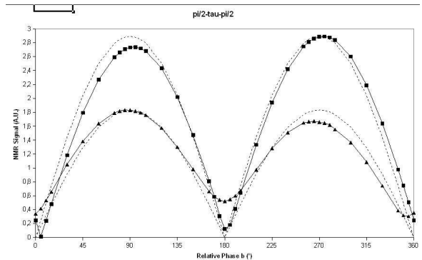
Figure 3: Amplitude of the NMR signal of 10 ml of water after two \pi/2 pulses versus the relative phase \beta of the two pulses. Continuous line (■ \text{NMR}_1 ) is obtained in a high a homogeneous magnetic field, large dashed (▲ \text{NMR}_2 ) line in a less homogeneous field. Fine dashed lines correspond to f(\beta) = G|\sin \beta| normalized to the maximum NMR signal in each case.
