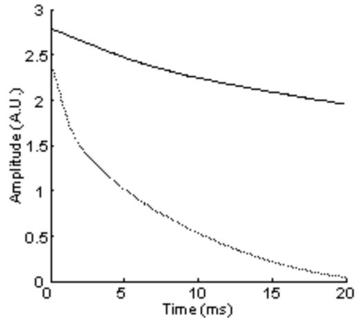
Figure 1: NMR signal (FID) of 10 ml of water after one \pi/2 pulse. Continuous line is obtained in a high homogeneous magnetic field ( \Delta B_0/B_0 = 2.0 \cdot 10^{-8} ) and dashed line in less homogeneous field ( \Delta B_0/B_0 = 2.7 \cdot 10^{-7} ).
