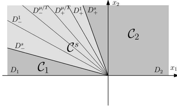
Figure 1: The cones \mathcal{C}_1, \mathcal{C}^s, \mathcal{C}_2 .
