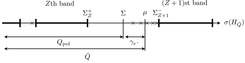
FIGURE 1. Decomposition \bar{Q} = Q_{\text{pol}} + \gamma_{e^-} for not too strong a positively charged nuclear defect ( \nu \geq 0 ).
