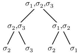
FIGURE 1. Skeleton of the 2-covering of B_4^+ of Example 2.5: a depth 2 binary tree displaying the inclusions between the generating sets of the successive submonoids.
