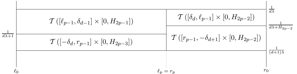
FIGURE 5. “Blow-up” of the relevant part of \Omega_\alpha for even q , 1/2 < \alpha < 1/\lambda .
