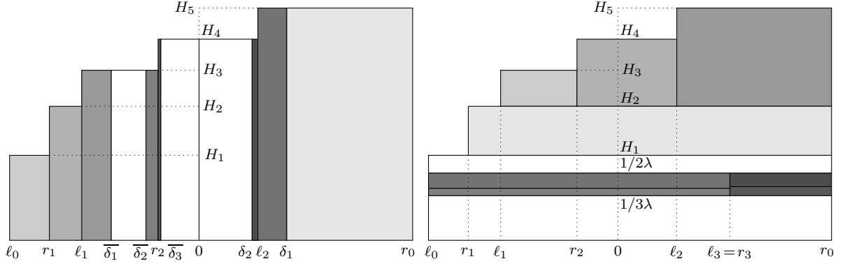
FIGURE 3. The natural extension domain \Omega_\alpha (left) and its image under \mathcal{T}_\alpha (right) of the \alpha -Rosen continued fraction (\overline{\delta_n} = -\delta_n) ; here q = 6 , \alpha = 0.53 , d_p(\ell_0) = 2 , d_p(r_0) = 3 .
