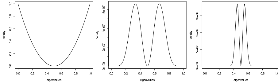
Figure 1: Theoretical eigenvalue distribution for (n = 2, k = 2) , (n = 2, k = 10) and (n = 2, k = 100) .
