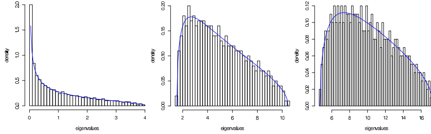
Figure 3: Empirical and limit measures for (n = 500, k = 500) , (n = 500, k = 1000) and (n = 500, k = 5000) .
