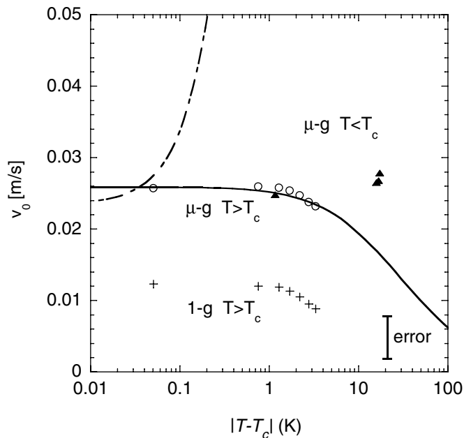
FIG. 6. Initial jet velocity v_0 as a function of temperature ( T > T_c , \mu -g, circles; T > T_c , 1g, crosses; T < T_c , \mu -g triangles). The full ( T > T_c ) and dashed ( T < T_c ) lines are calculated from Eq. (1).
