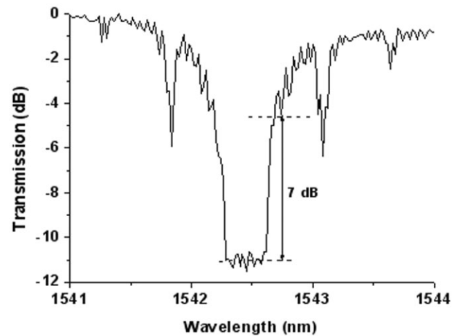
Figure 2 Measured transmission spectrum for 5-mm-long uniform filter
