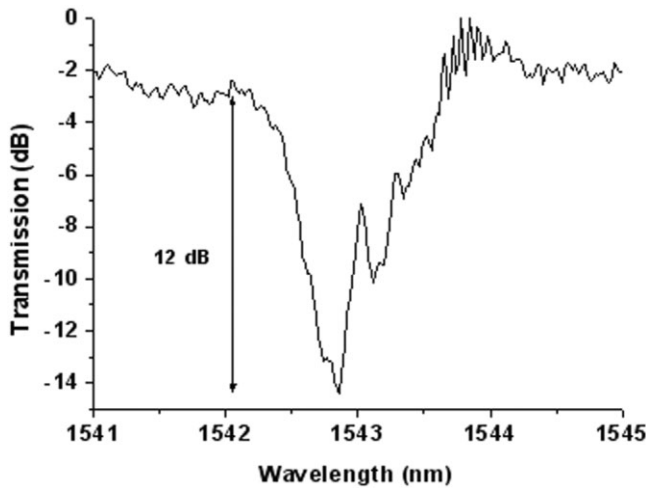
Figure 4 Transmission spectrum for the half-apodized filter
