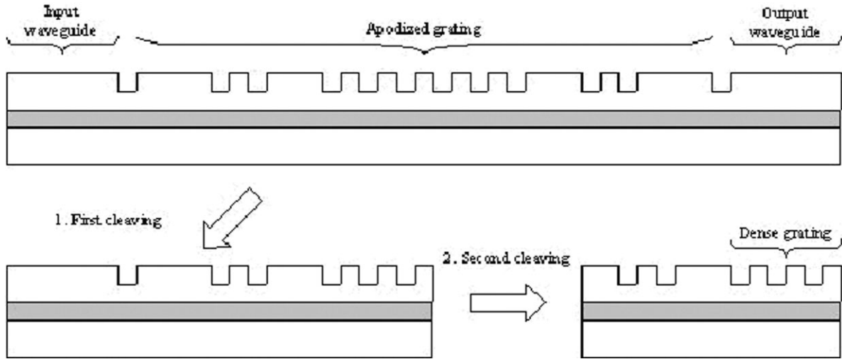
Figure 3 Schemes of the entire and cleaved apodization filters tested
