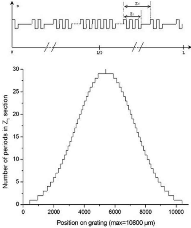
Figure 1 Sampled grating design: schematic view (top) and Gaussian distribution of Z_1 sections
