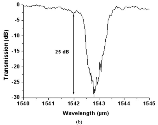
Figure 5 Measured transmission spectra of apodized Bragg grating filter (half), with light injection from the dense grating side (b) and the other side (a)
