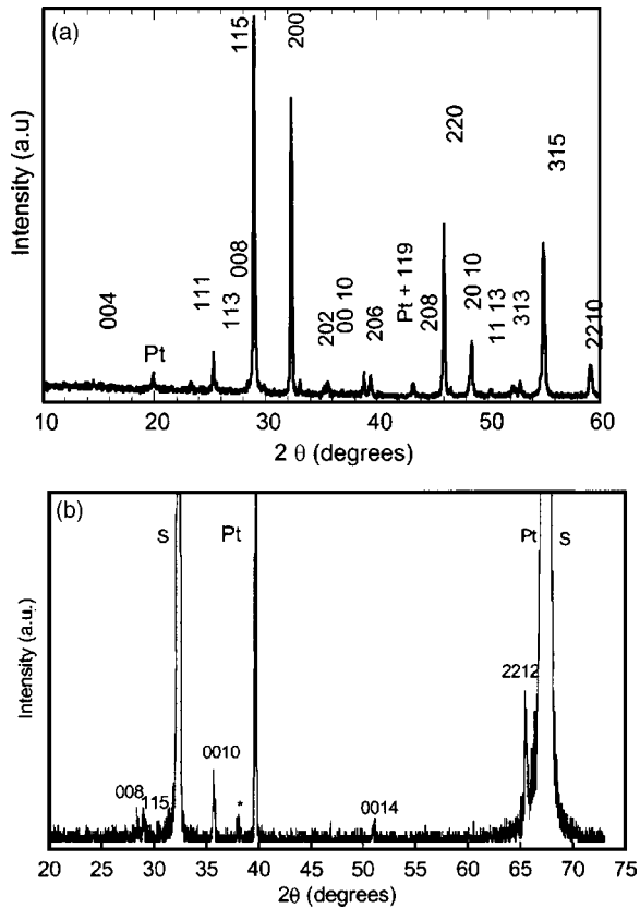
FIG. 1. X-ray diffraction patterns for \text{SrBi}_2\text{Nb}_2\text{O}_9 films grown (a) on Pt-coated Si (sample A) and (b) on (110)Pt epitaxially grown on (110) \text{SrTiO}_3 (sample B).
