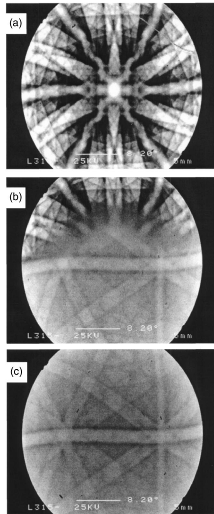
FIG. 2. Electron channeling pattern of the (110)Pt bottom electrode (a) and of the (116) \text{SrBi}_2\text{Nb}_2\text{O}_9 film B. (c) ECP of the median region is represented in (b). A schematic drawing of the bilayers epitaxially grown on (110) \text{SrTiO}_3 is given on the top of the figure.
