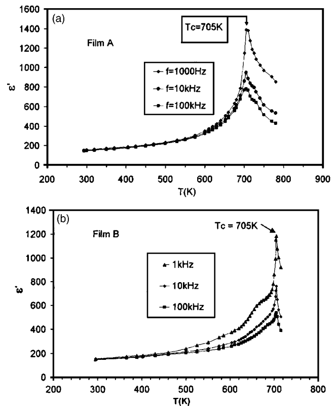
FIG. 5. Dielectric permittivity measurements vs temperature performed at 1, 10, and 100 KHz, for sample A (a) and sample B (b).
