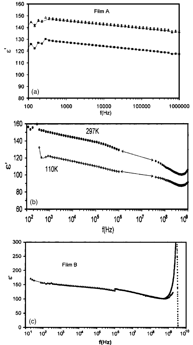
FIG. 7. Evolution of the dielectric permittivity \epsilon' vs frequency for samples A (a) and B [(b) and (c)]. Data recorded for several electrodes are reported for sample A (a). Measurements were performed for sample B at 297 and 110 K (b).
