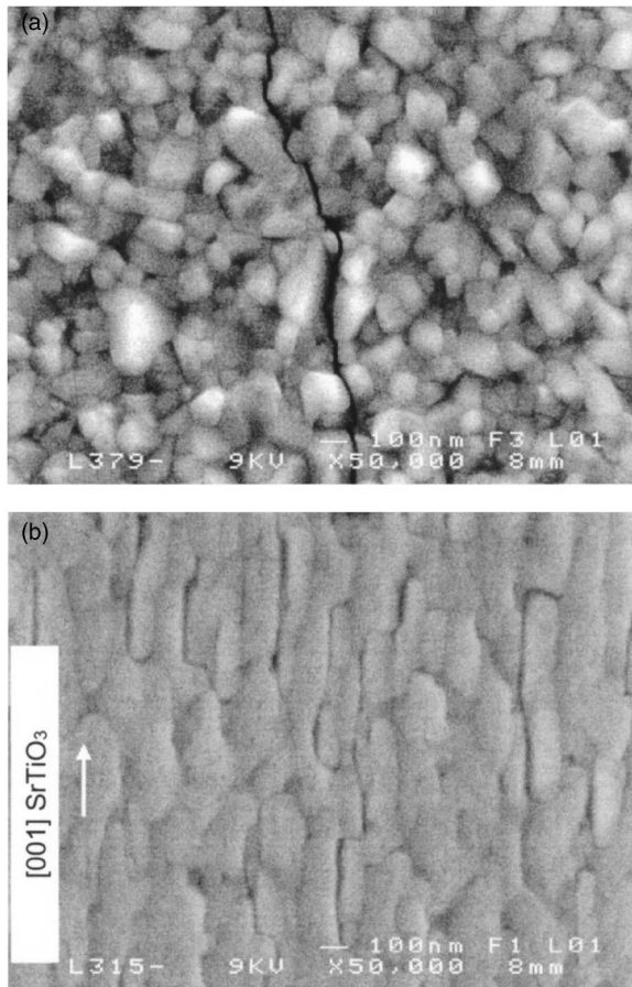
FIG. 3. Scanning electron microscopy observations of \text{SrBi}_2\text{Nb}_2\text{O}_9 films grown on Pt-coated Si [(a) sample A] and on (110)Pt epitaxially grown on (110)SrTiO 3 [(b) sample B].
