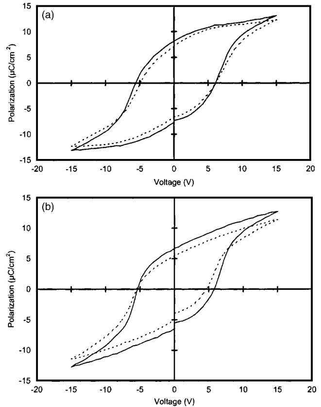
FIG. 4. Hysteresis loops recorded before (full line) and after (dotted line) fatigue tests for samples A (a) and B (b).
