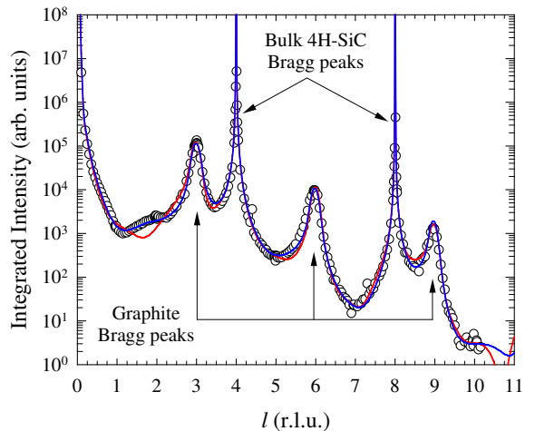
FIG. 2: (color on line) X-ray (00l) reflectivity data from 9 graphene layers grown on the 4H-SiC(000 \bar{1} ) surface. Bulk and graphite Bragg peaks are labelled. Blue line is the best fit structure with one reconstructed SiC bi-layer as described in the text. Red line is a fit with an extended reconstruction of two SiC bi-layers.
