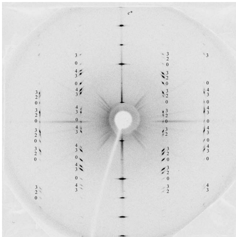
Figure 4 Precession diffraction pattern from the third SX plane (SX3) of the sample No. 1 (120° from SX1). The l index is as given in Fig. 2.
