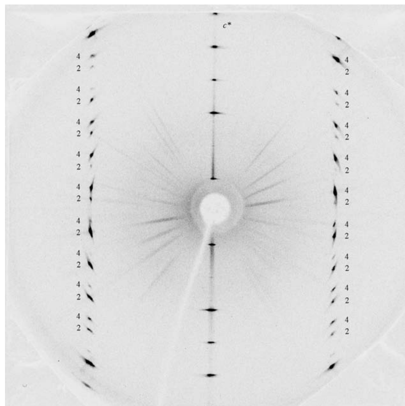
Figure 5 Precession diffraction pattern from an SD plane of the sample No. 1 (30° from SX3). The l index is as given in Fig. 2.
