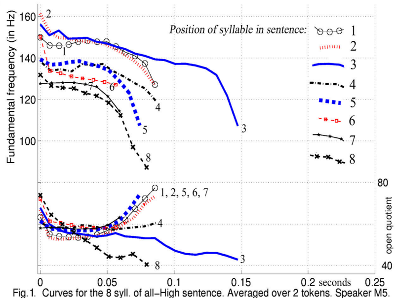
Fig. 1. Curves for the 8 syll. of all-High sentence. Averaged over 2 tokens. Speaker M5.
