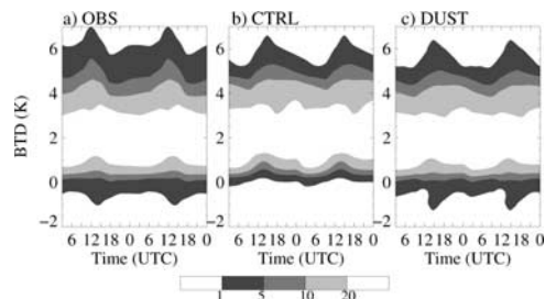
Figure 3. Bi-diurnal cycle of filtered BTD (K) distribution obtained from (a) the observations, and the 3–48 h forecasts with the (b) CTRL and (c) DUST simulations.
