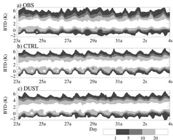
Figure 2. Time evolution of the BTD (K) distribution obtained from (a) the observations, and the 27–48 h forecasts of the (b) CTRL and (c) DUST simulations. The time axis is indicated by the day; a, August; s, September.
