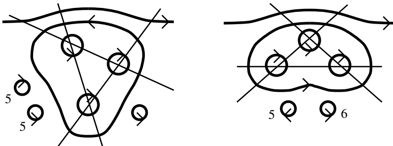
FIGURE 7. Two curves of degree seven with different triple locks
