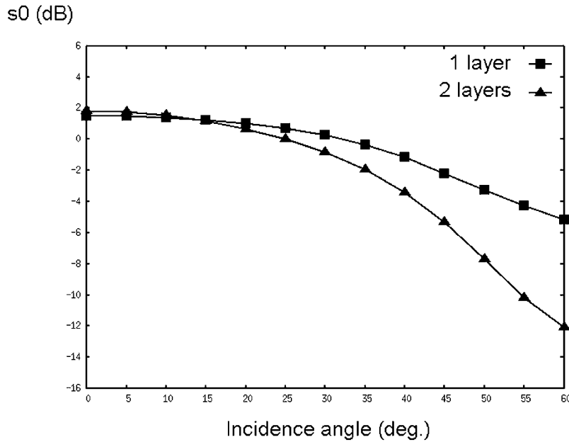
Figure 4. One-layer (squares) and two-layer (triangles) backscattering power of radar-bright regions with respect to the SAR incidence angle.
