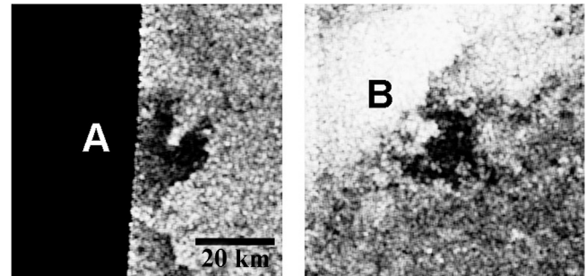
Figure 5. Radar-dark spots (left) A at incidence angle 30^\circ and (right) B at incidence angle 23^\circ in Ta flyby SAR data.
