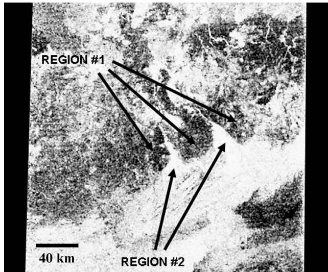
Figure 2. Radar-bright study site located at 50.92°N, 79.35°W.
