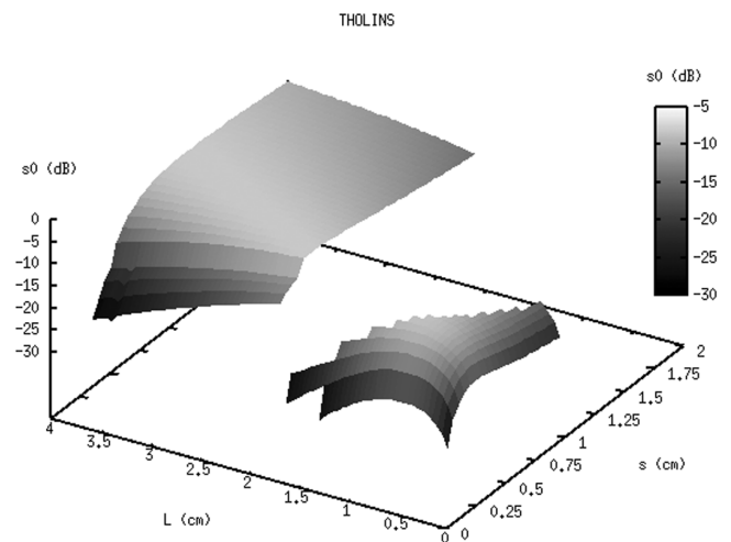
Figure 3. Backscattered power of a single layer of tholins with respect to roughness parameters \sigma and L at an incidence angle \theta = 30^\circ .
