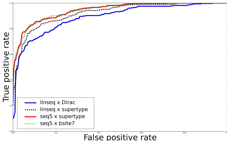
Figure 1: ROC curves on the pooled five folds of the SYFPEITHI+LANL benchmark.
