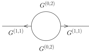
Figure 3. Single diagram contributing to C(\mathbf{q}, t, t) in the s -state, at minimal order with respect to the external momentum \mathbf{q} . The expressions for the propagators are given in (63).
