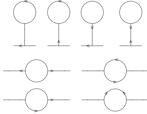
Figure 2. One-loop graphs which renormalise the correlation function in the s -state.
