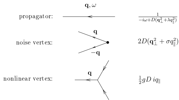
Figure 1. Propagator, noise vertex, and nonlinear vertex used in the perturbation expansion for the driven lattice gas.
