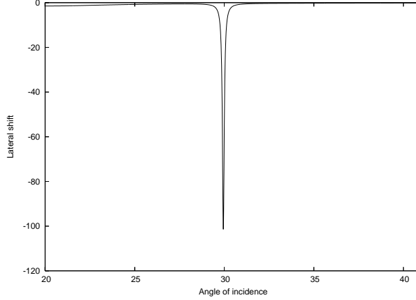
Figure 2: Lateral shift \frac{\Delta}{\lambda} [1, 7] versus the angle of incidence for \epsilon_1 = 12 , \mu_1 = 1 , \epsilon_2 = -5 and \mu_2 = -0.5 and d = 0.6\lambda . The angle above which the field is evanescent in the LHM is 27.16^\circ .
