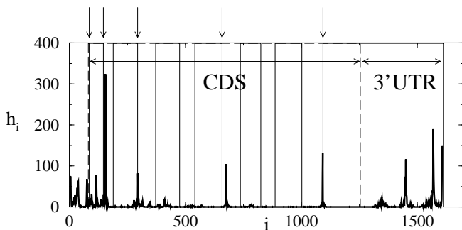
FIG. 5: Histogram of the thermodynamic boundaries (think line) of the Human cDNA encoding for the interleukin enhancer binding factor 2 (ILF2) protein with Gene Bank entry NM_004515. The thin vertical lines denote exon-exon (solid) and CDS-UTR (dashed) boundaries. The arrows indicate the exon-exon boundaries detected by the melting analysis.
