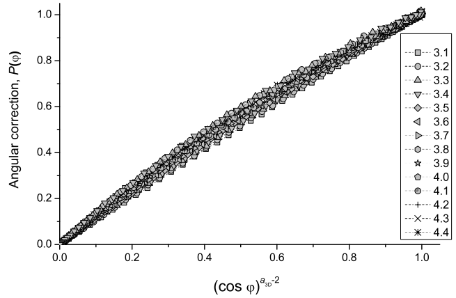
Figure 4. Same as figure 3, except the horizontal axis that is (\cos \varphi)^{a_{3D}-2} . The scattering observed in Figure 3 appears to be significantly reduced.
