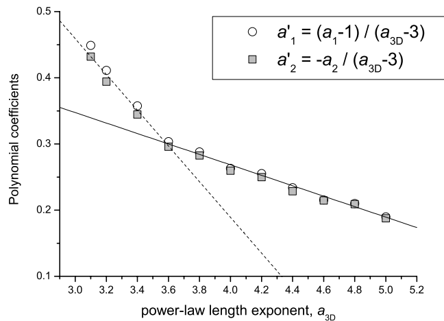
Figure 5. Dependency of the reduced polynomial coefficients a'_1 (= (a_1 - 1)/(a_{3D} - 3)) and a'_2 (= -a_2/(a_{3D} - 3)) with the power law exponent a_{3D} . The parameters a_1 and a_2 are defined in equation (5).
