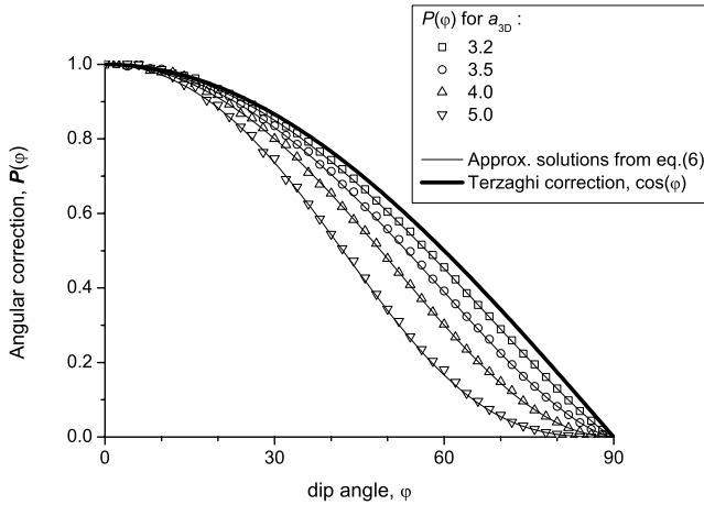
Figure 3. Angular correction for a fracture of dip \varphi . Fracture centers are chosen so that an equivalent horizontal fracture necessarily transects the core (i.e., the distance between the fracture center and the core axis is less than (l - d)/2 , with l and d the fracture and core diameter, respectively). The symbols correspond to power law fracture size distribution with exponents a_{3D} of 3.2 (squares), 3.5 (circles), 4.0 (triangles) and 5.0 (inverted triangles). The thin lines are approximated solutions calculated with equation 6. The thick solid line is the Terzaghi correction P(\varphi) = \cos\varphi .
