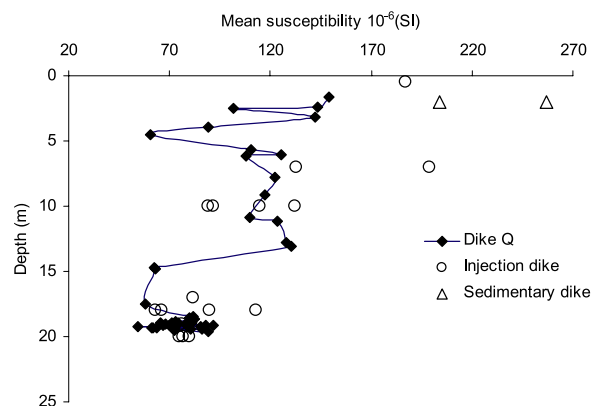
Figure 6. Variations of the mean susceptibility values with depth below the upper gypsum layer. Susceptibility values increase unmonotonously upward along Dike Q and all others dikes. Diamonds, Dike Q; circles, injection dikes; triangles, sedimentary dikes.
