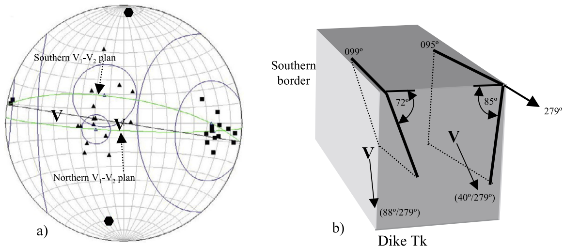
Figure 12. Analysis of the flow directions in Dike Tk, following Moreira et al. 's [1999] procedure. (a) Lower-hemisphere, equal-area projections of V_1 - V_2 planes. Principal axes V_1 and V_2 are marked by squares and triangles, respectively; the ellipses are 95% confidence ellipse. Each plane is projected by the two mean vectors. Diamonds represent poles to the planes, and the solid line represents the dike strike. The flow vector V is found by taking 90° backward to the stereogram center from the intersection point between those planes and dike strike. Generally, the mean vectors are associated with large 95% confidence ellipses, but with downward flow direction. (b) Schematic illustration of V_1 - V_2 planes along the borders of Dike Tk.
