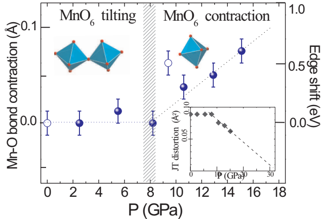
Figure 3: Relative changes in Mn - O distance in the pressure range 0 to 15.3 GPa. The plain circles are obtained by increasing the pressure and the open circles correspond to the release. The curve in the inset gives an estimation of the JT distortion defined by (\sigma_{JT})^2 = (\sqrt{1/6} \cdot \sum |R_i - R|)^2 and predicts a suppression of the distortion above 30 GPa
