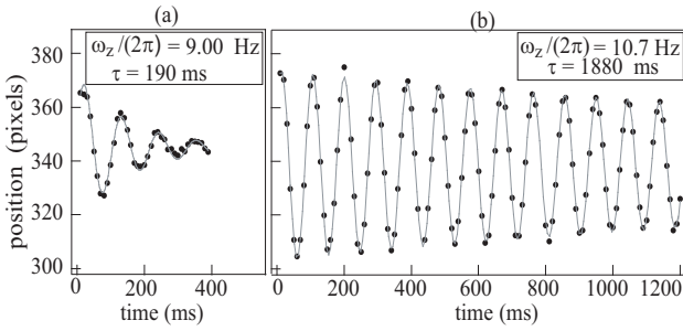
FIG. 3: Center of mass position vs time for negative DC current (a) and AC current (b). Dots are measurements and the solid line is a fit to the function Z(t) given in the text. The dramatic increase in damping time in the AC trap illustrates the strong reduction of the roughness.
