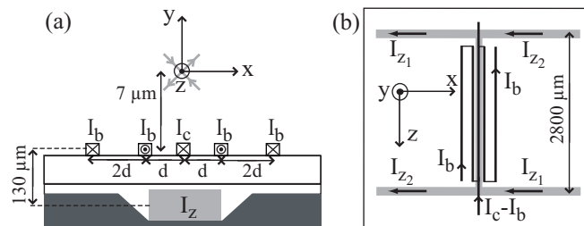
FIG. 1: Side (a) and top (b) view representations of the atom chip. The first wafer (dark grey) contains 15\ \mu\text{m} thick wires (grey). On the second wafer (white), a five wire structure creates the atomic guide whose roughness is studied ( d = 2.5\ \mu\text{m} ). The lengths in the drawings are not to scale.
