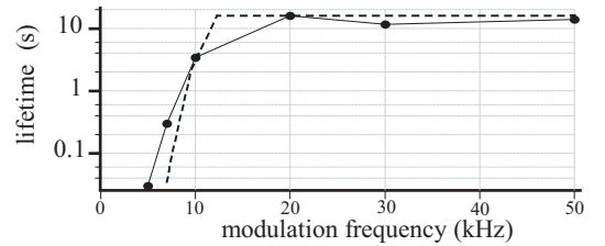
FIG. 4: Modulation frequency dependence of the atomic lifetime in the modulated trap (dots). The dashed line represents the result of Monte Carlo calculations with a transverse magnetic field of 150 mG for both x and y directions. The lifetime in the unmodulated trap is typically 10 s.
