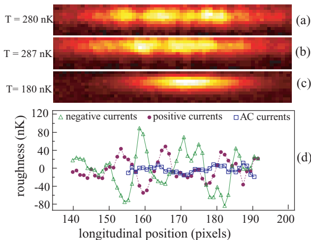
FIG. 2: (Color on line). Absorption images of a thermal cloud for negative DC (a), positive DC (b), and AC currents (c), respectively. In (d), the potential roughnesses are extracted from longitudinal profiles using Maxwell-Boltzmann's distribution. The pixel size is 6 \mu\text{m} .
