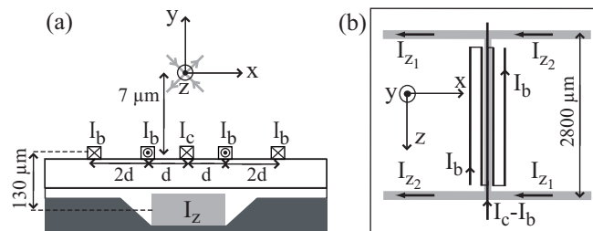
FIG. 1: Side (a) and top (b) view representations of the atom chip. The first wafer (dark grey) contains 15 \mu\text{m} thick wires (grey). On the second wafer (white), a five wire structure creates the atomic guide whose roughness is studied ( d = 2.5 \mu\text{m} ). The lengths in the drawings are not to scale.
