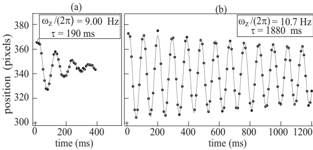
FIG. 3: Center of mass position vs time for negative DC current (a) and AC current (b). Dots are measurements and the solid line is a fit to the function Z(t) given in the text. The dramatic increase in damping time in the AC trap illustrates the strong reduction of the roughness.
